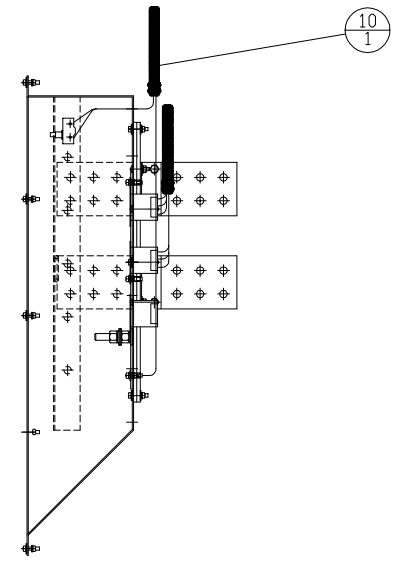
RIGHT SIDE VIEW DOOR REMOVED
