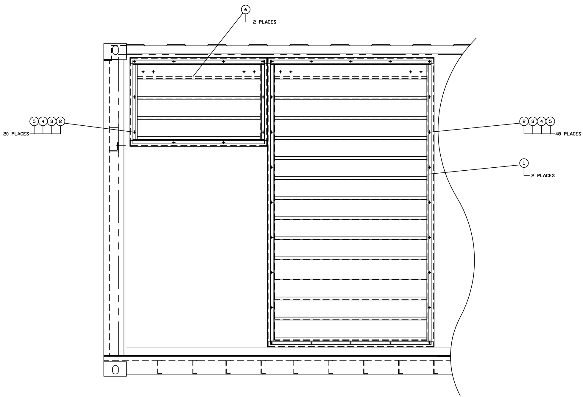
PARTIAL - CONTAINER SIDE
