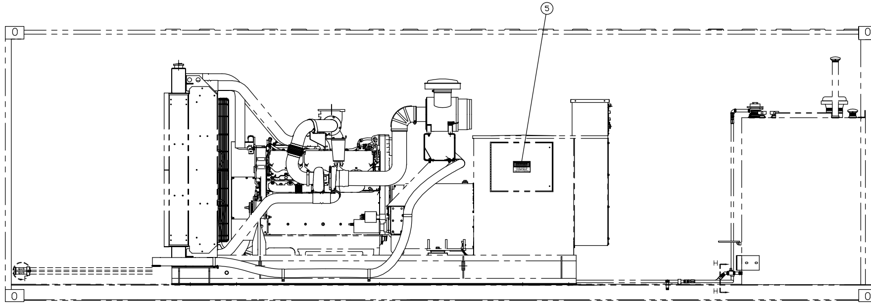
RIGHT SIDE VIEW OF CONTAINER
