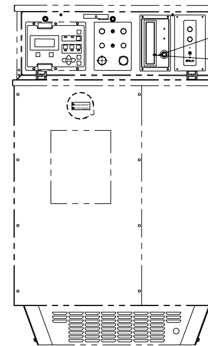
SECTION G-G AT B-7 SCALE 2=1
