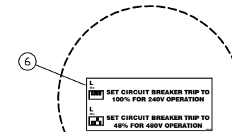
VIEW J AT E-3 SCALE 5=1
